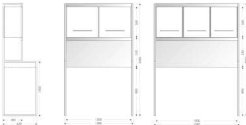
Studioline D Boceto lateral
